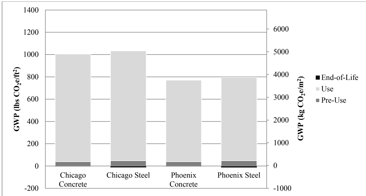
Figure 4.8 – GWP normalized by gross floor area over a 60-year lifespan for commercial buildings separated by phase
