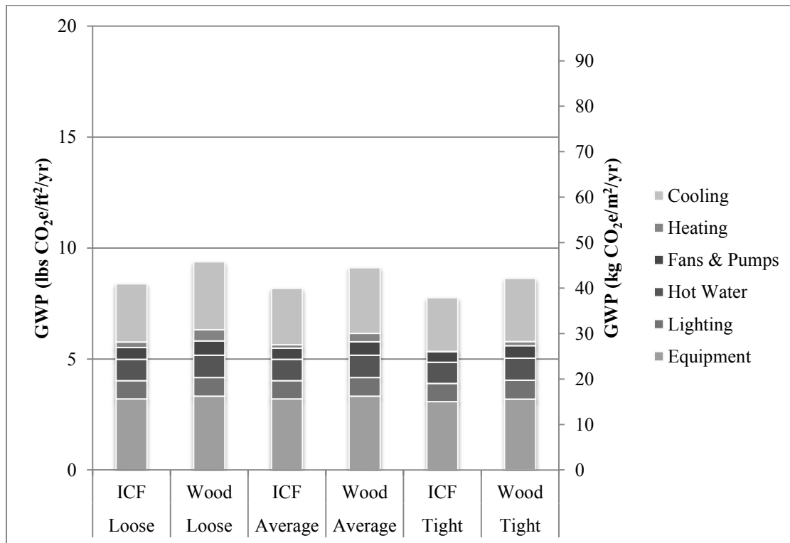
Figure 3.9 – GWP associated with annual energy use and normalized by gross floor area for the single-family houses in Phoenix, separated by air tightness and energy end-use
