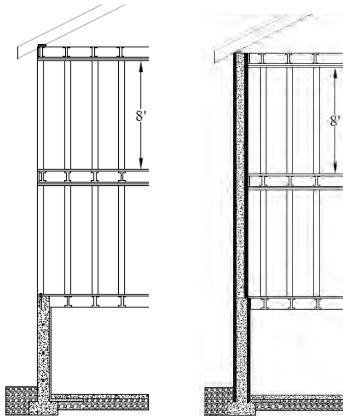
Figure 3.2 – Structural design of the light-frame wood and ICF single-family houses for Phoenix
