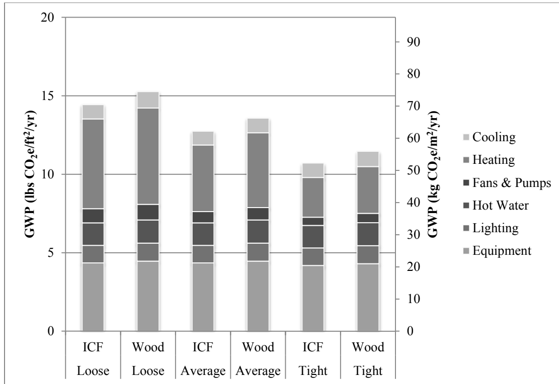
Figure 3.8 – GWP associated with annual energy use and normalized by gross floor area for the single-family houses in Chicago, separated by air tightness and energy end-use
