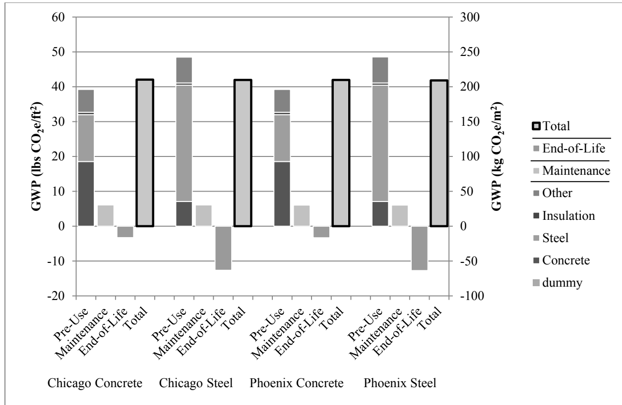
Figure 4.5 – Embodied GWP normalized by gross floor area and separated by material and phase for the commercial buildings
