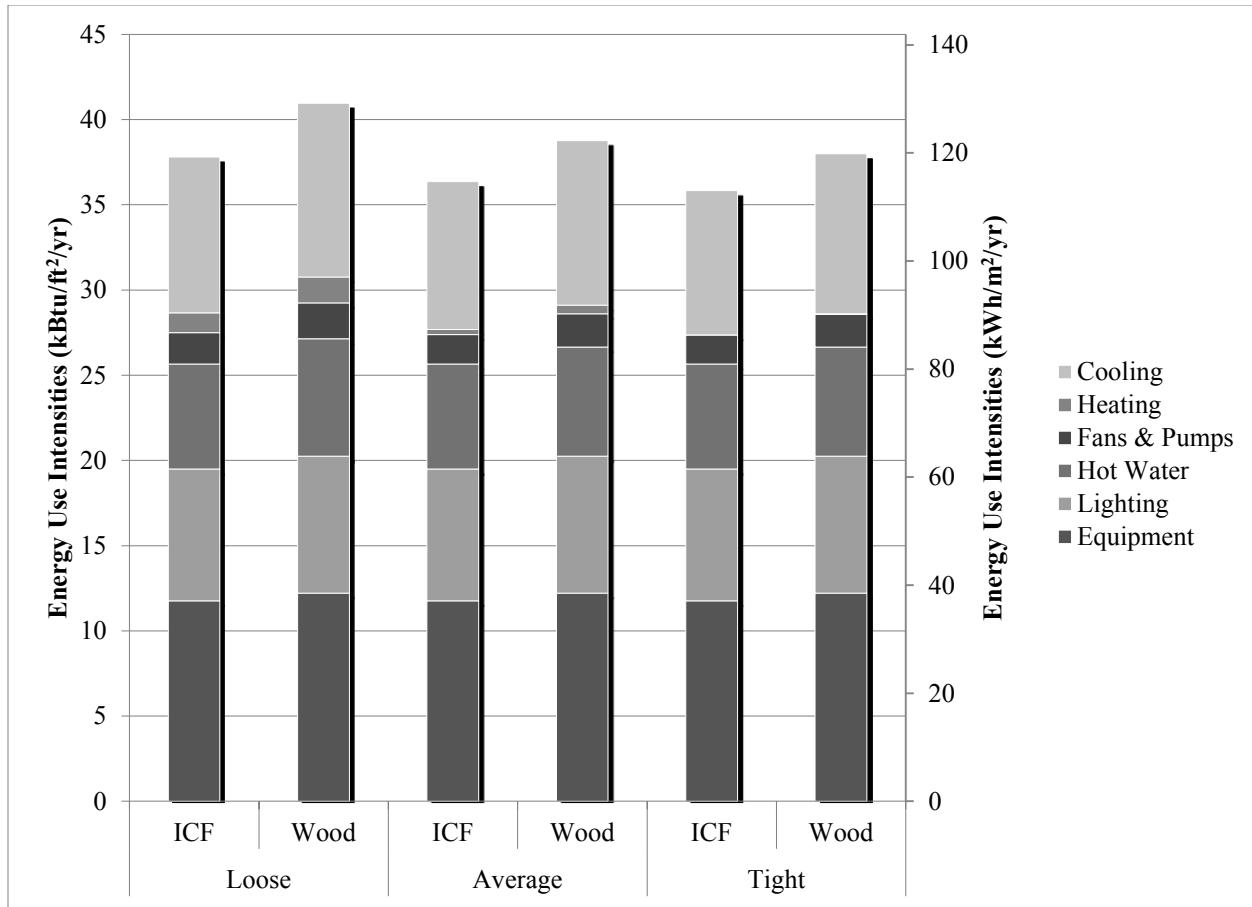
Figure 3.23 – Annual energy use intensities normalized by gross floor area for the multi-family houses in Phoenix, separated by air tightness and energy end-use.
