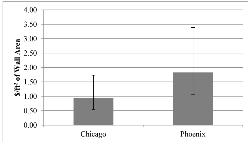
Figure 3.12 – Present value of energy savings over the 60-year lifetime of the ICF wall compared to wood construction for 2,400 ft 2 (223 m 2 ) single family house
