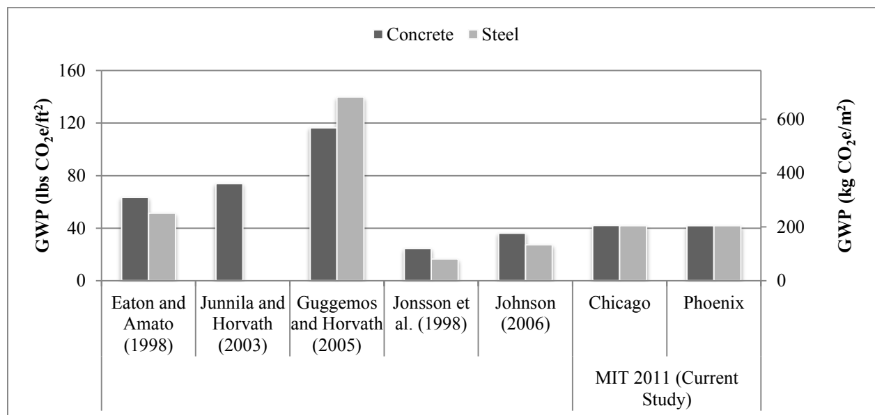
Figure 5.2 – Comparison of embodied global warming potential of commercial office buildings normalized by floor area (Hsu 2010)
