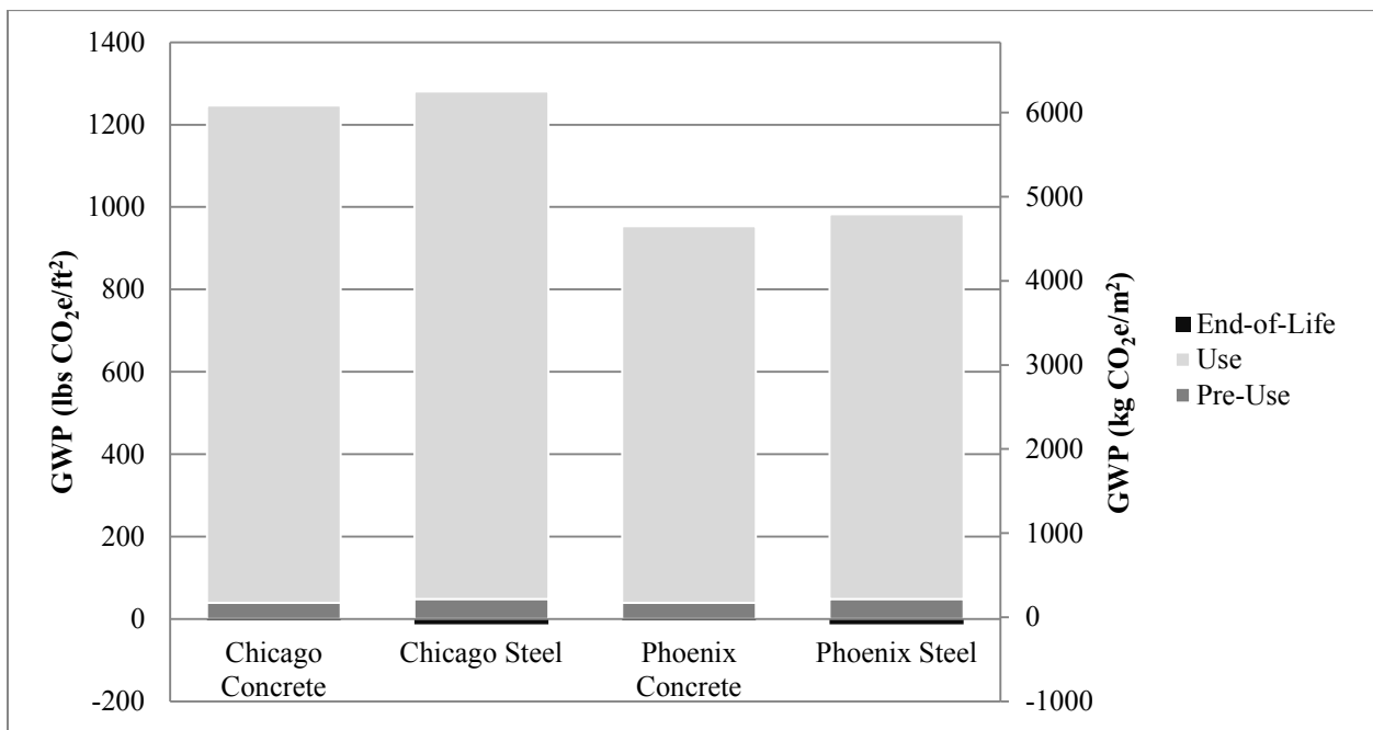
Figure 4.9 – GWP normalized by gross floor area over a 75-year lifespan for commercial buildings separated by phase
