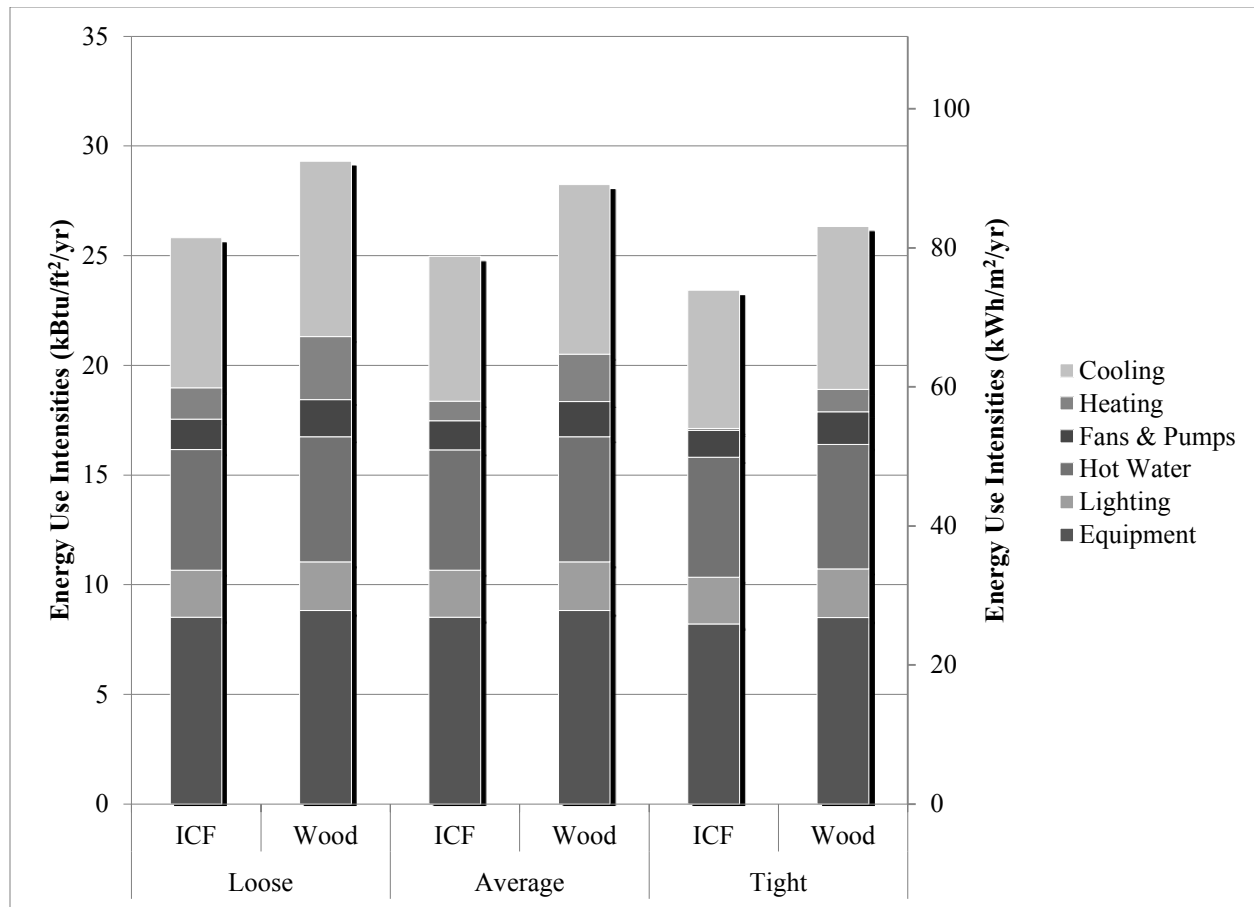
Figure 3.7 – Annual energy use intensities normalized by gross floor area for the single-family houses in Phoenix, separated by air tightness and energy end-use
